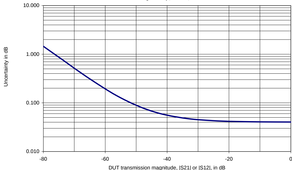
Transmission magnitude uncertainty R&S®FSH4/R&S®FSH8
