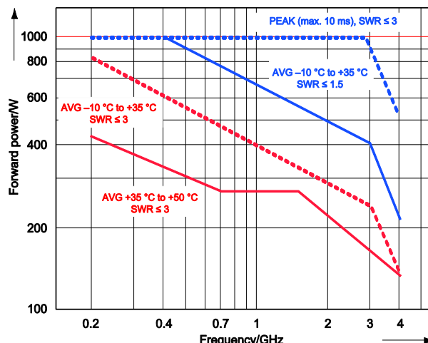
Power-handling capacity.
